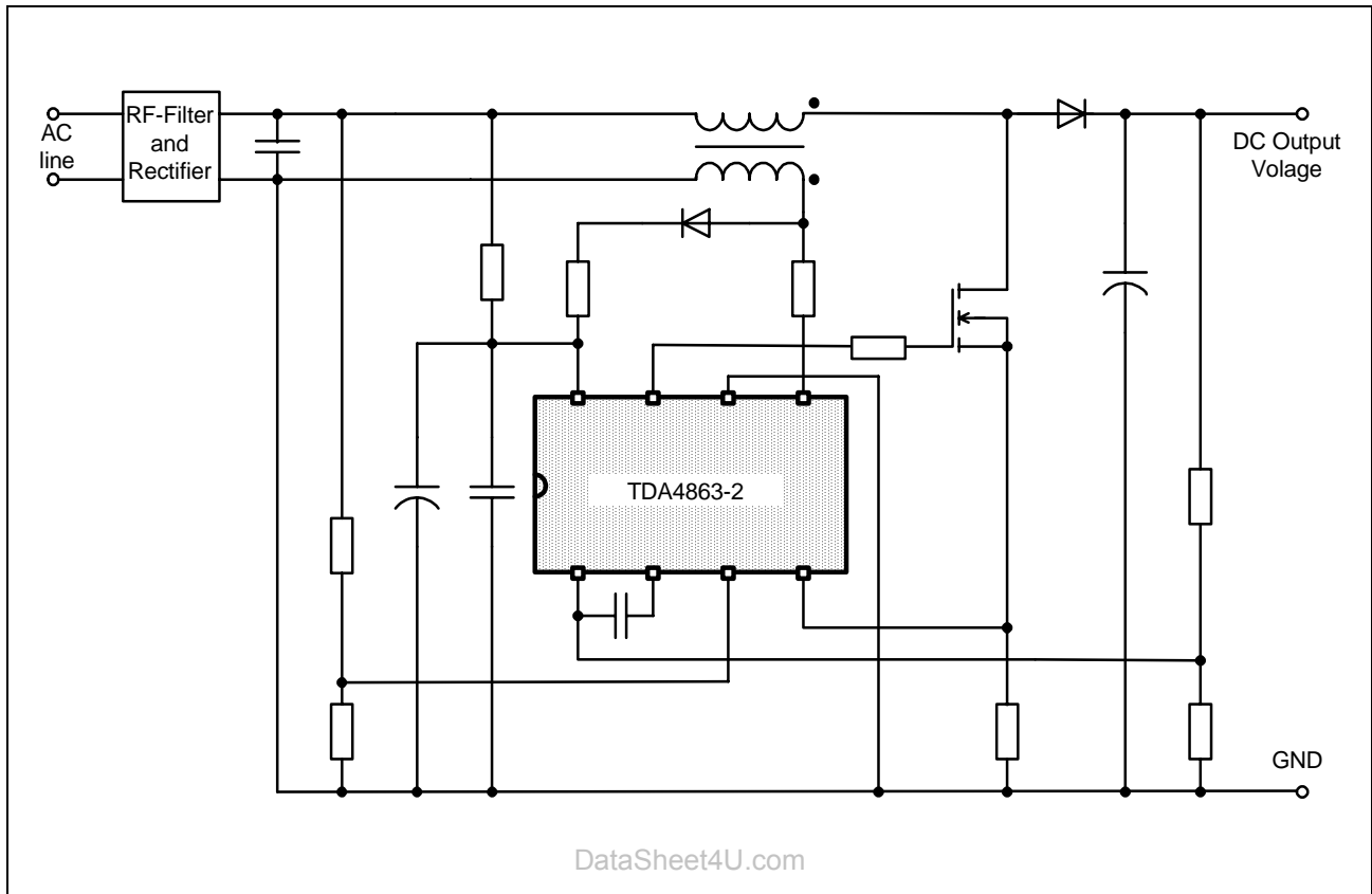
Figure 1 Typical application
