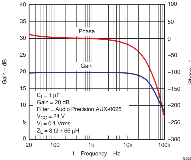
GAIN/PHASE vs FREQUENCY (PBTL)
